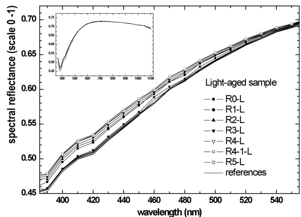
Fig. 8. Spectral curves of light-aged samples for different numbers of aging cycles applied. For comparison, the corresponding curves of the reference sample are plotted as plain lines. Insert: Overview of entire wavelength range. The most significant changes are in the blue-green range of the visible part of the spectrum
