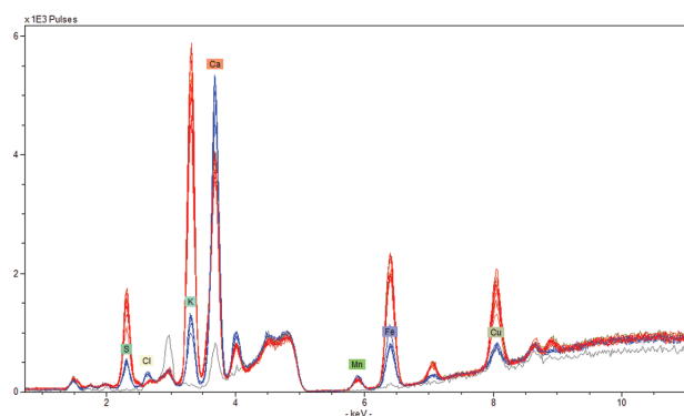
Fig. 2. XRF spectra of paper spots from Quinta Europa map (good condition, 5 spots) and Septima Asiae Tabula (poor condition, 10 spots); the grey line shows the air spectrum, which contains peaks that are artifacts from materials in the instrument. Peak labels are shown directly above peaks in the Quinta Europa map spectra
