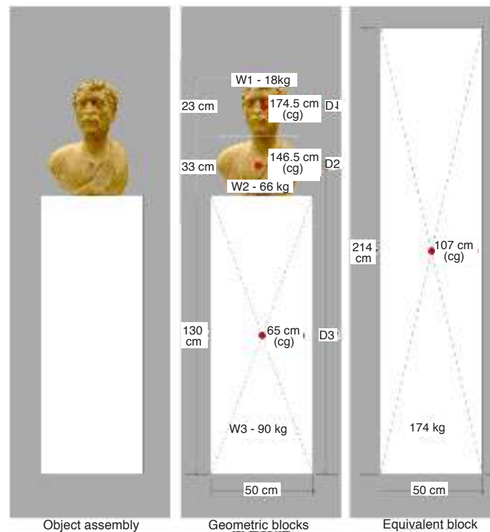
Figure 4. Determining the equivalent block of an object assembly, in this case a sculpture and a pedestal combination.
