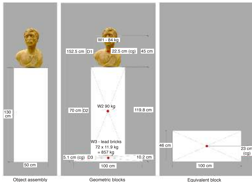
Figure 5. Looking at the system's new equivalent block, the cg has been lowered to 23 cm by adding 857 kg and increasing the base by 50 cm. NOTE: The center of gravity must be calculated for the added weight mass, in this case lead. Stacking the weight too high will cause the mass to become unstable.
